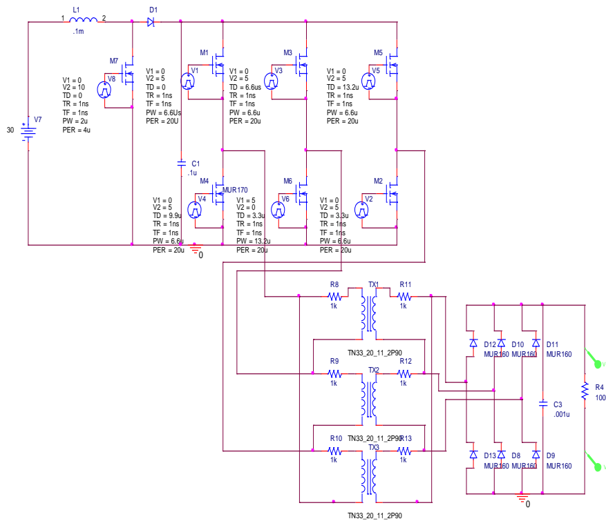
Fig 5.Simulated circuit diagram
