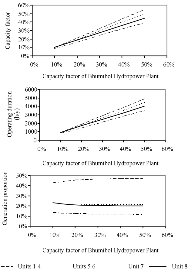
Figure 4. Determinations of capacity factor, operating duration, and generation proportion of the Bhumibol hydropower plant
