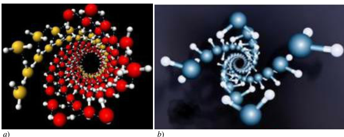
Figure 6: Spiral structures of water nanocrystals in carbon nanotubes according to computer simulations (Bai et al. , 2006) (diameter of nanotubes 1.35–1.90 nm; pressure 10–40000 atm; temperature -23 °C): a) – a general view of the crystal structure of water in nanotubes, b) – the inner wall of the structure of water.
