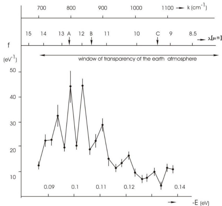
Figure 3: The NES-spectrum of deionized water (chemical purity – 99,99 %; pH – 6,5–7,5; total mineralization – 200 mg/l; electric conductivity – 10 \mu S/cm): the horizontal axis shows the energy of the H...O hydrogen bonds in the associates – E (eV); the vertical axis – the energy distribution function – f ( eV^{-1} ); k – the vibration frequency of the H–O–H atoms ( cm^{-1} ); \lambda – wavelength ( \mu m )
