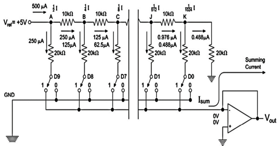
Figure 5: 2R-R circuit with 10 input
