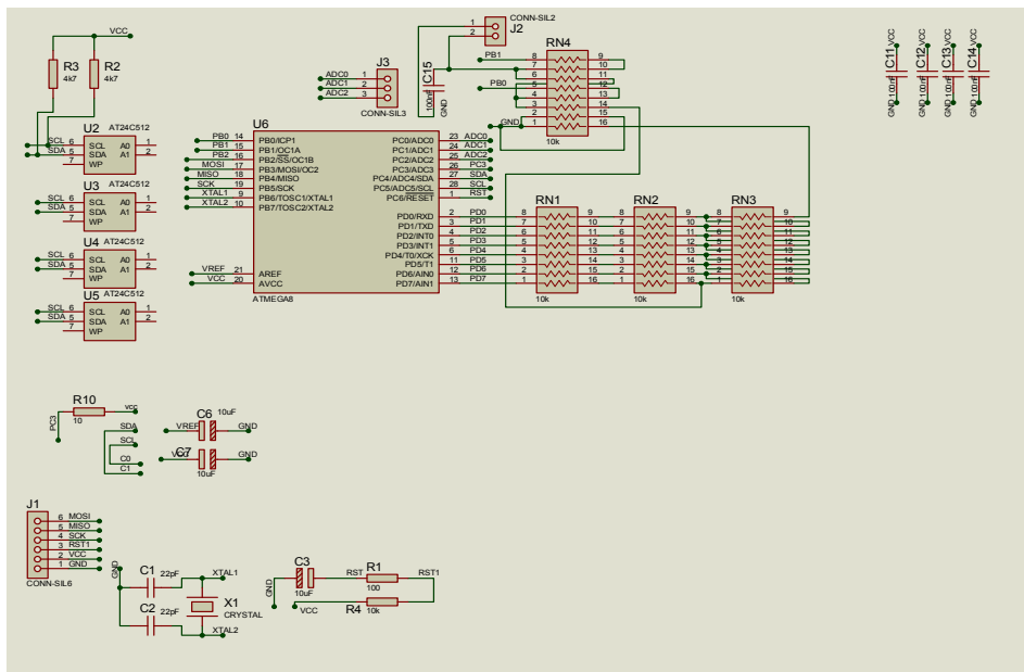
Figure 2: Microcontroller circuit
