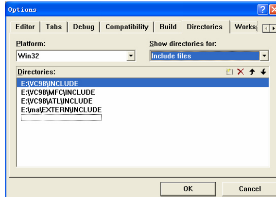
Figure 1. Add "E:\ma\EXTERN\Include"
