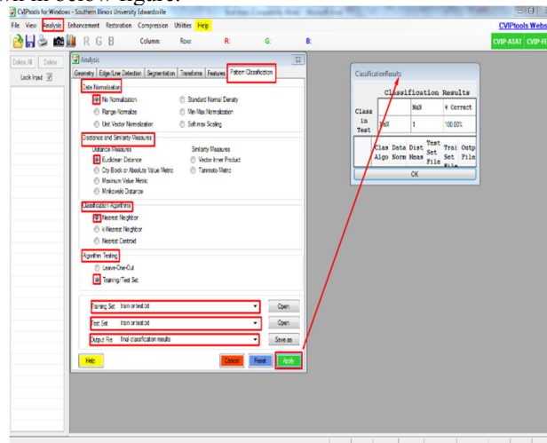
Figure 4: Pattern Classification
