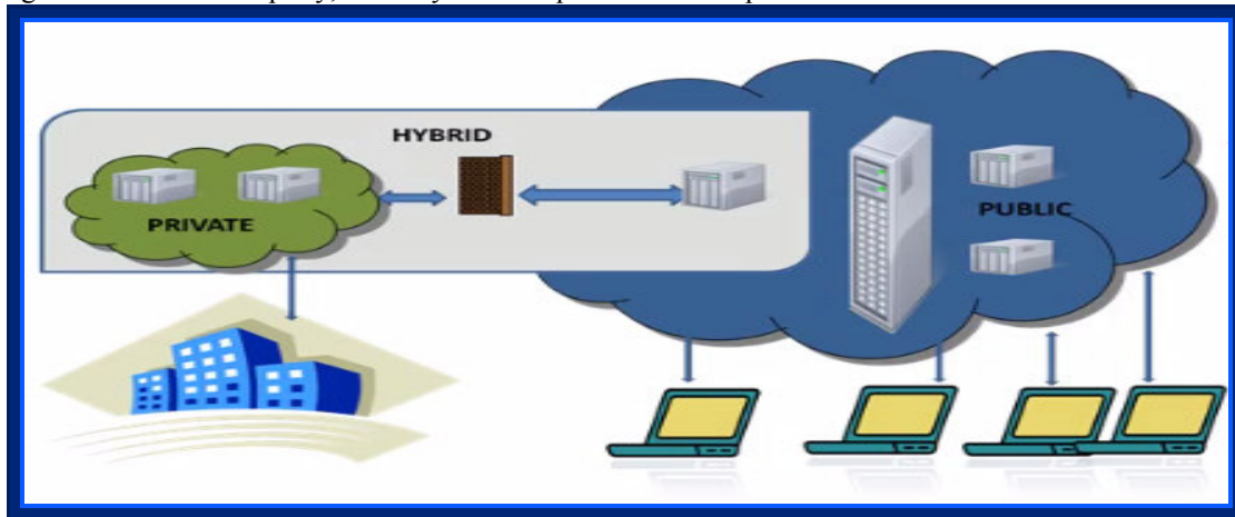
Fig.7 Deployment models
