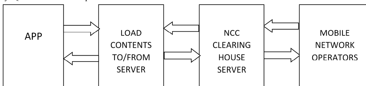
Figure 6 3 tier Architecture
