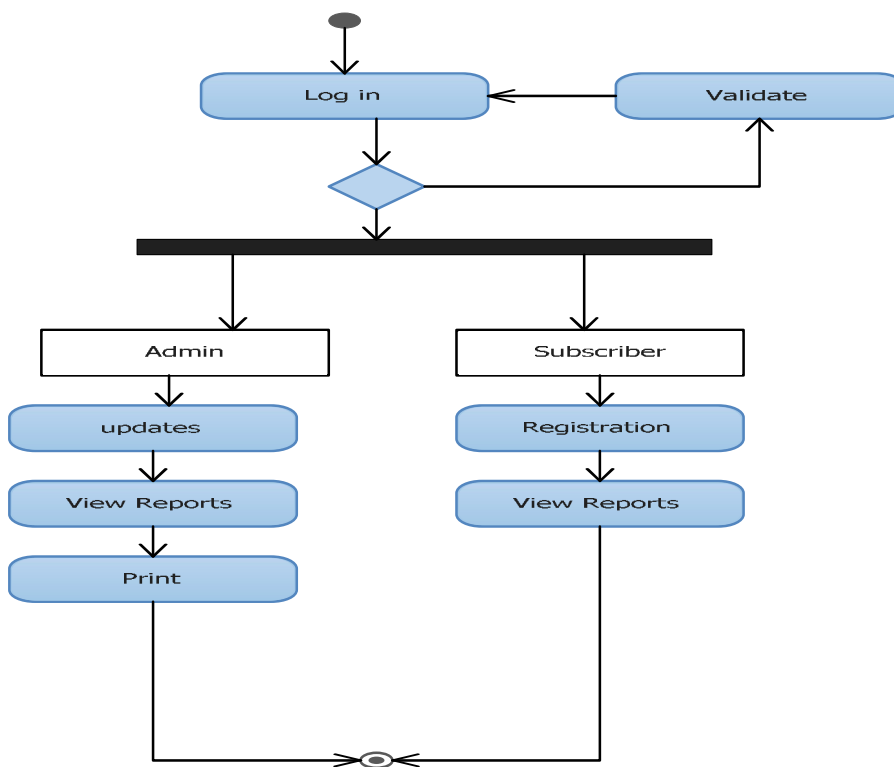
Figure 4 Activity Diagram
