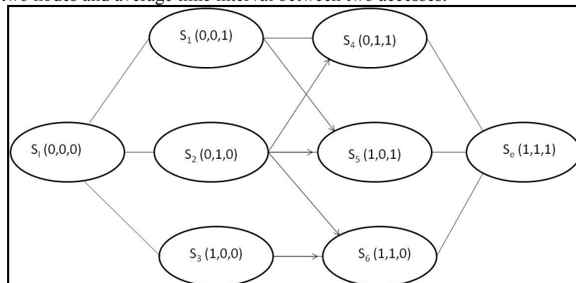
In state transition graph of content diffusion suppose that one state is S and user i already access the content state S_m .
