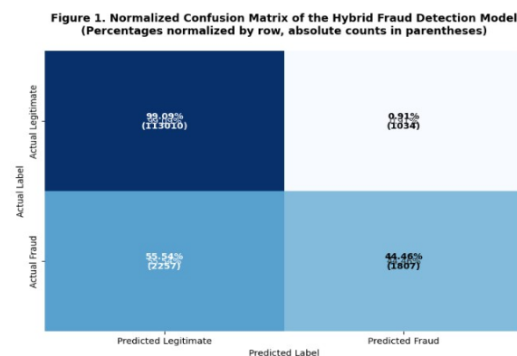
Figure 5 Confusion Matrix
