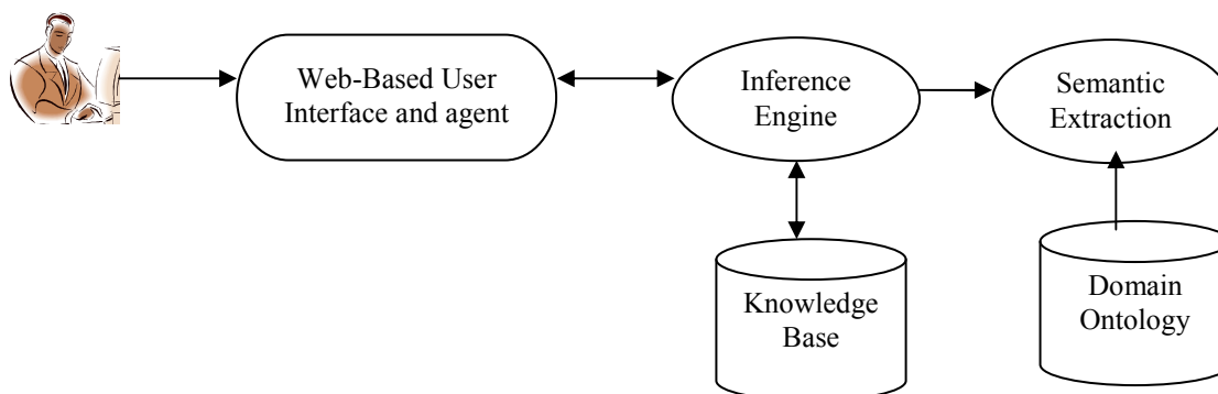
Figure 7: System Architecture
