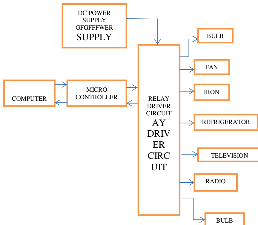
Figure.2: Block Diagram of the designed system
