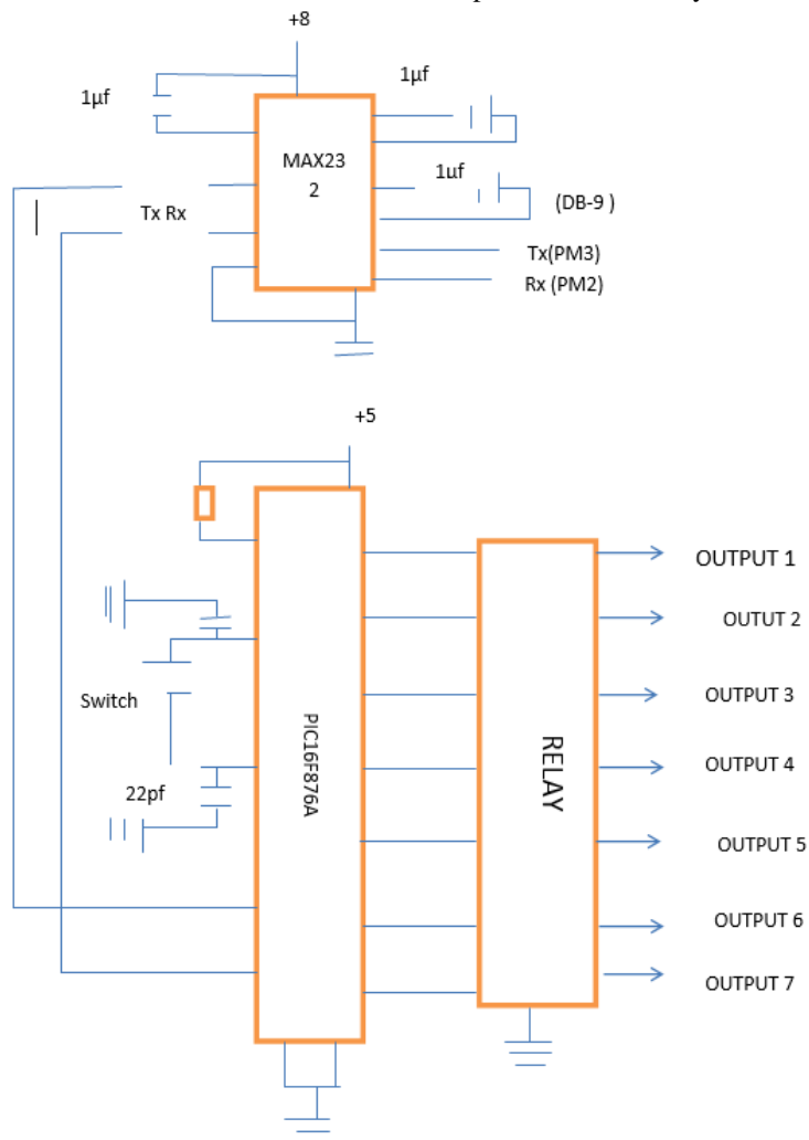
Figure 4: Main component circuit analysis
