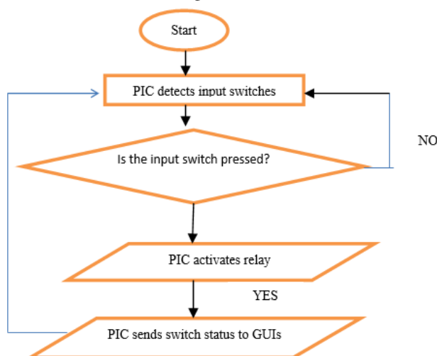
Figure 6: Flow chart showing PIC- GUI communication
