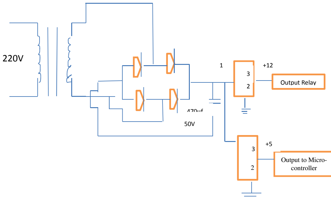
Figure 3: Power supply regulation circuit
