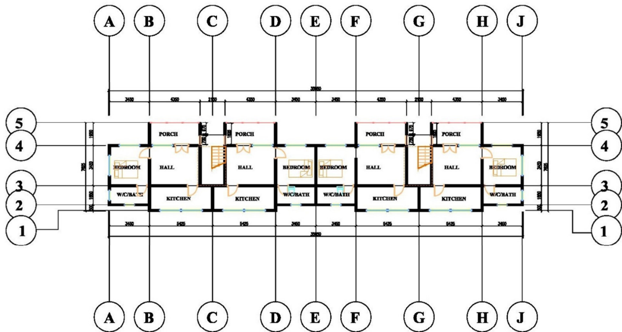
Proposed Ground Floor plan of Faculty accommodation at PDM University
