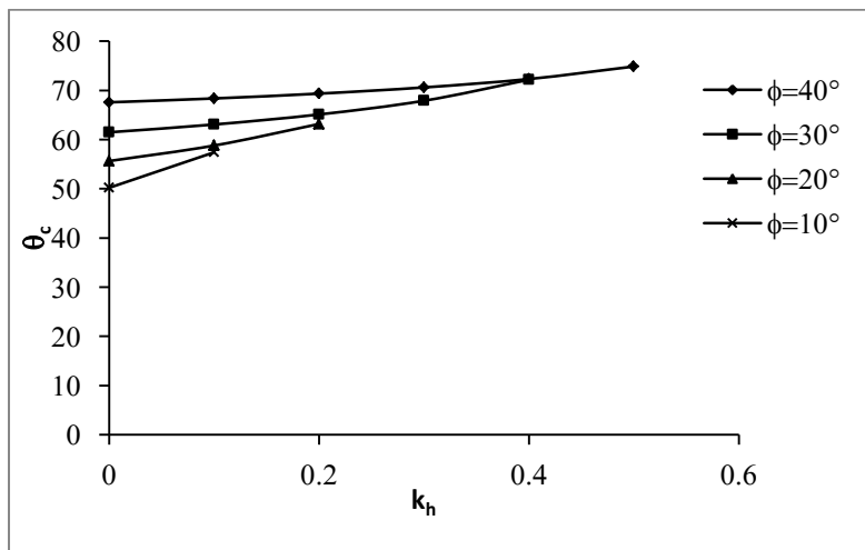
Fig.11.Variation critical wedge angle ( \theta_c ) with k_h for k_v=k_h/2 , \delta=\Phi/2 , \gamma = 18 \text{ kN/m}^3 , c=10 \text{ kN/m}^2 , c_a = 8 \text{ kN/m}^2 , q = 15 \text{ kN/m} , H=10 \text{ m} , a=20^\circ
