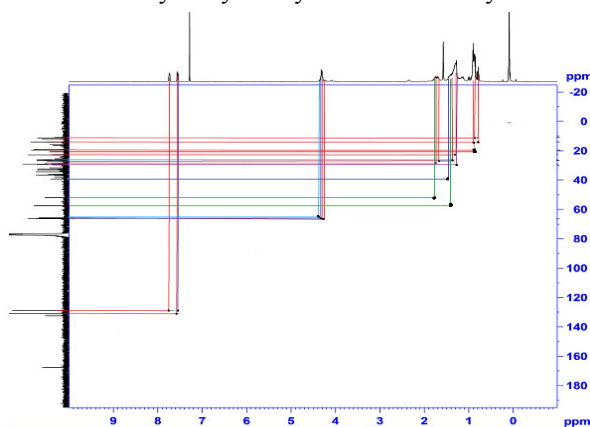
Figure 9: HETCOR of Hydroxy methyl taraxastene Ethyl benzoate in \text{CDCl}_3
