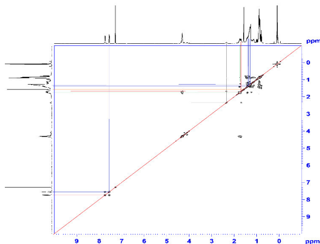
Figure 7: ^1\text{H} - ^1\text{H} COSY of Hydroxy methyl taraxastene Ethyl benzoate in \text{CDCl}_3
