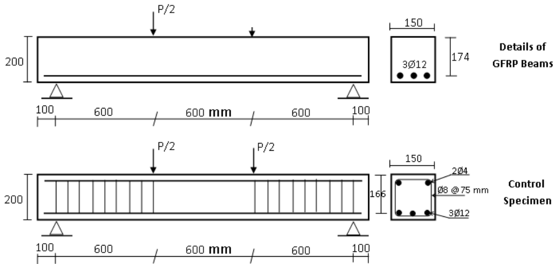
Figure 1 :Typical Geometry and Reinforcement Details for Beams
