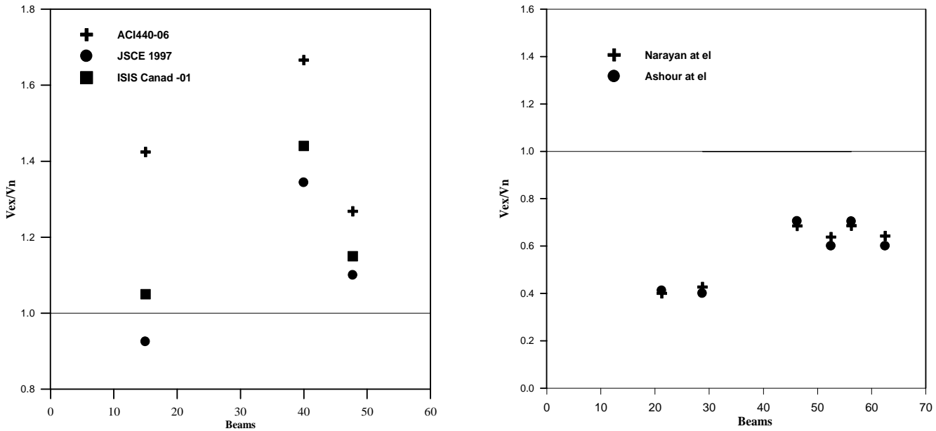
Figure 9 :Experimental to Calculated Shear Strength of FRP-Reinforced Concrete Beams
