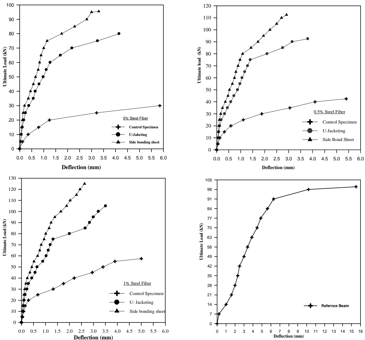
Figure 8 : Load – Deflection Curve for Beams Strengthened with CFRP Laminate
