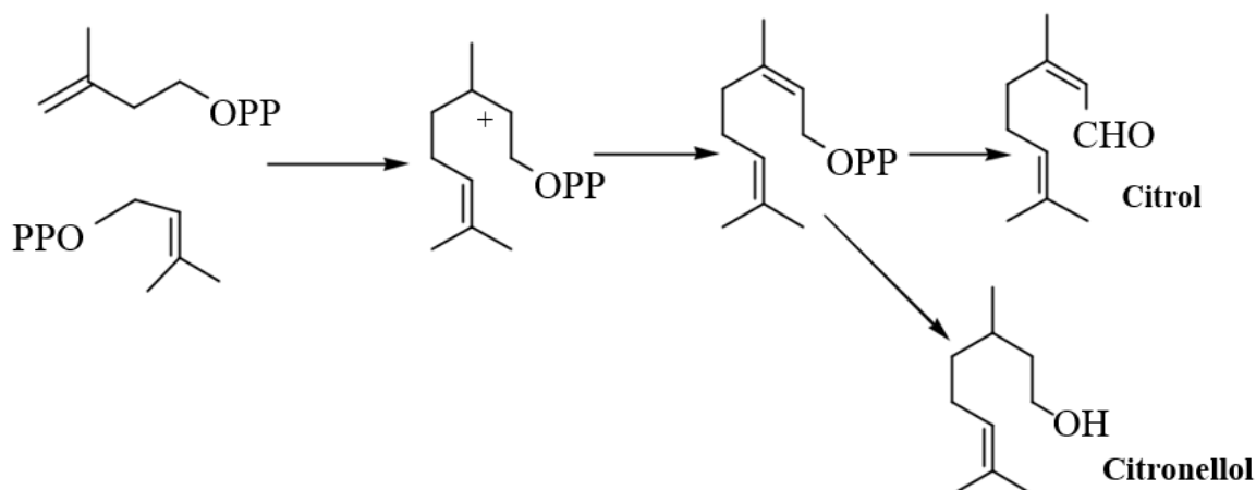
Scheme 3: Biogenesis of Monoterpenes
