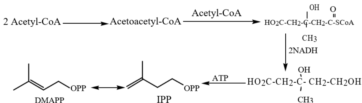
Scheme 2: Biogenesis of IPP (the Mevalonate path way)
