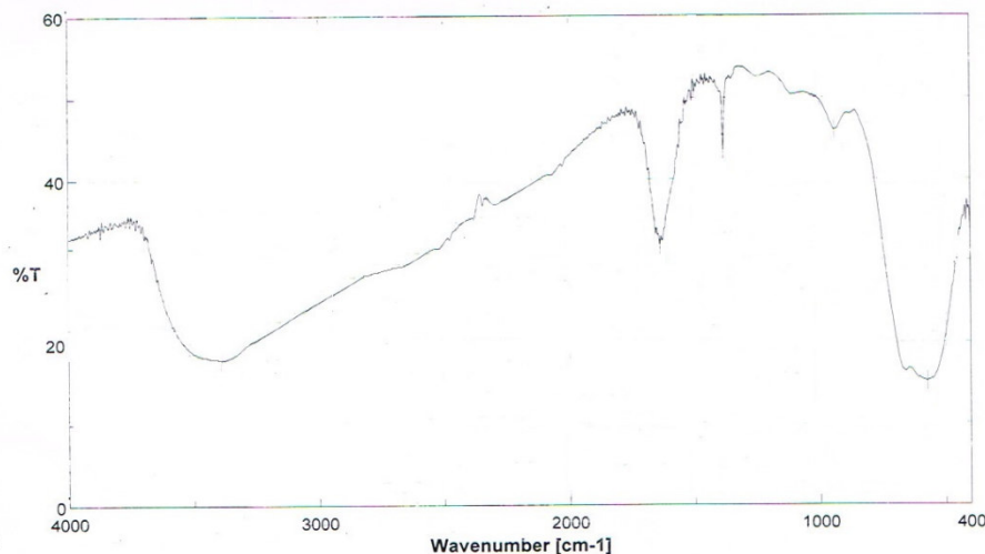
Figure (4): Represents FTIR spectrum of antimony doped tin oxide by (3wt%).
