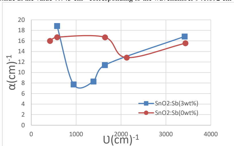
Figure (6): the absorption coefficient by the wavenumber function of pure SnO 2 and Sb doped SnO 2 powder by (3wt%) .
