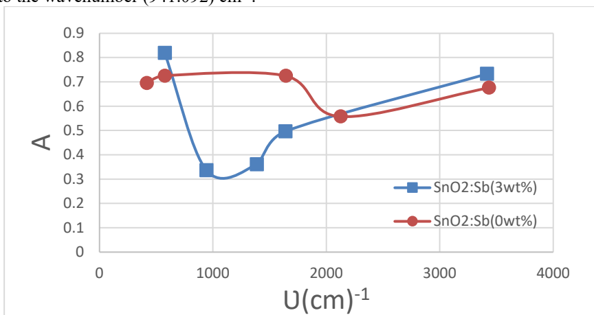
Figure (5): the absorbance by the wavenumber function of pure SnO 2 and Sb doped SnO 2 powder by (3wt%) .
