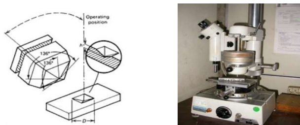
Figure 5. Hardness Testing Equipment and Diamond pyramid test indenter schematic for Vickers test and its indentation
