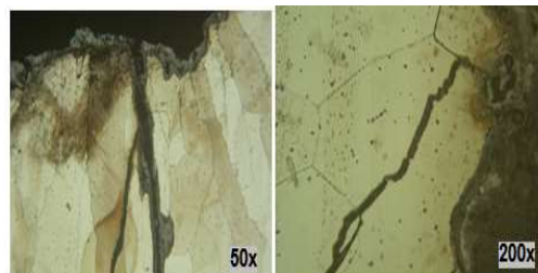
Figure 19. Macro photo of the Holding Magnet TYPE LS50 C sample with 50x and 200x magnification.
