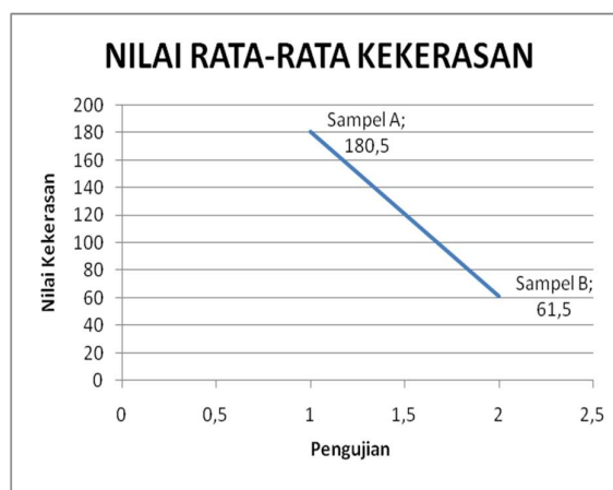
Figure 24. Graph of Average Value of hardness test on CuZn (ring) on Holding Magnet Type LS50.
