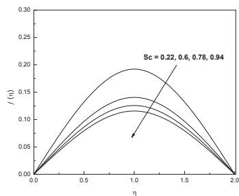
Figure 11: Velocity profiles for different values of Sc
