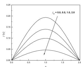
Figure 15: Velocity profiles for different values of f_w
