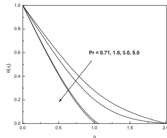
Figure 8: Temperature profiles for different values of Pr
