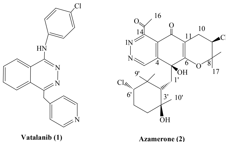
Fig. 1 Structures of Vatalanib and Azamerone.
