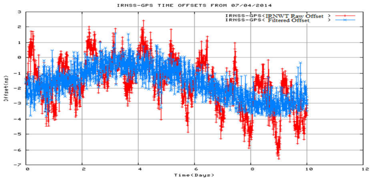
Figure 6 IRNSS-GPS Time offset data from 07/04/2014
