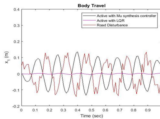
Figure 13: Body travel for random road disturbance
