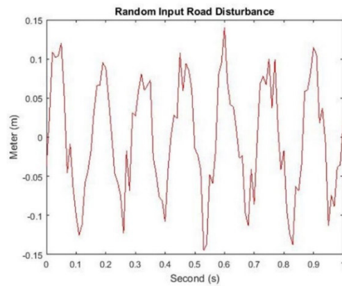
Figure 3: Random road disturbance
