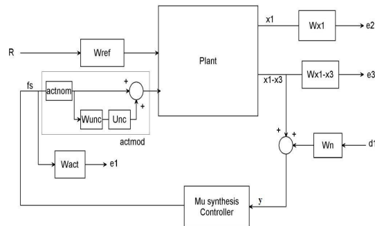
Figure 6: Active suspension system with \mu - synthesis controller system interconnections block diagram The output or feedback signal y is
