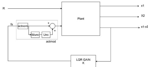
Figure 7: State variable feedback configuration
