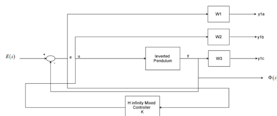
Figure 2 The inverted pendulum with H \infty mixed sensitivity controller
