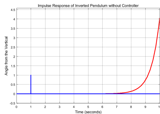
Figure 6 Impulse response of inverted pendulum without controller
