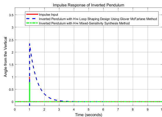
Figure 10 Impulse response
