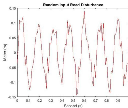
Figure 2: Random road profile
