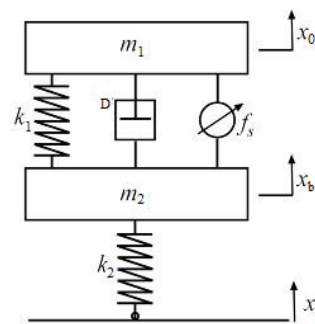
Figure 1: Quarter model of active suspension system.
