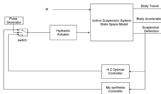
Figure 3: Active suspension system with H2 optimal and \mu - synthesis controller's system block diagram The switching system switch in micro seconds. The hydraulic actuator model is a second order transfer function defined as:
