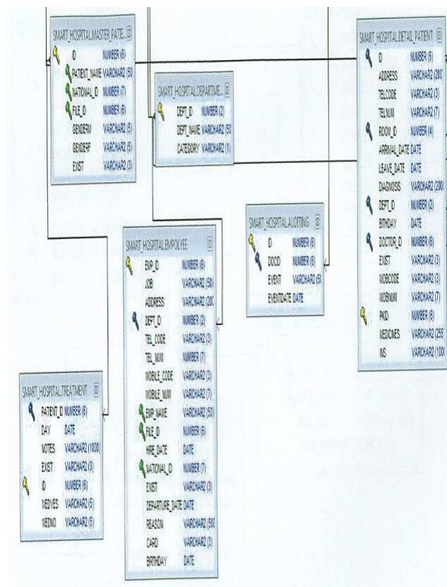
Figure 3c: Smart Hospital Schema 3
