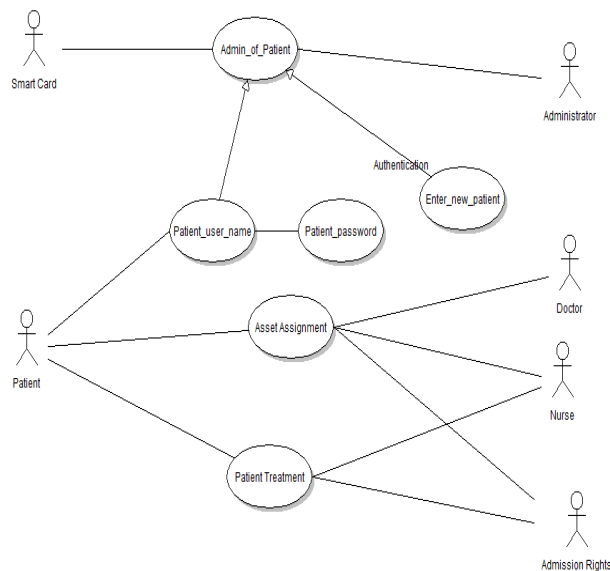
Figure 1a: Use-case diagram
