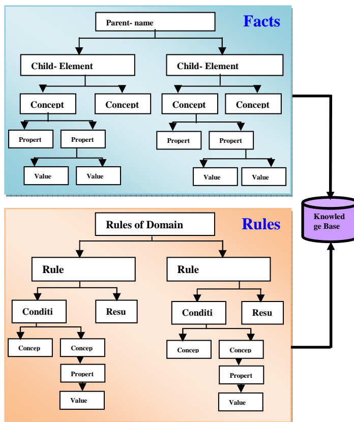
Figure1b: Overall knowledge structure
