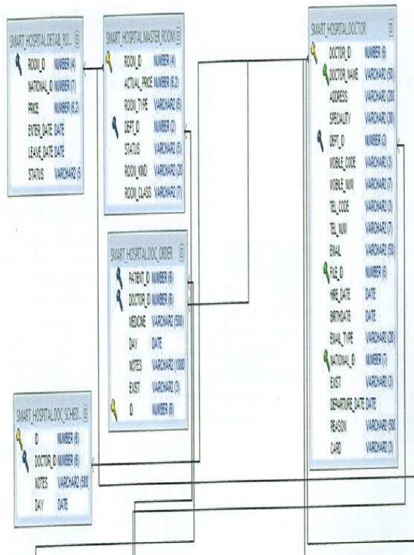
Figure 3a: Smart Hospital Schema 1.
