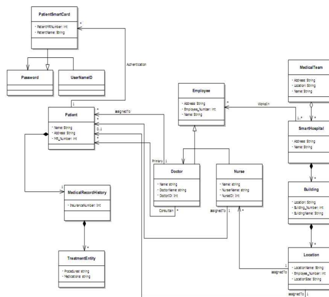
Figure 6(a): Class diagram for patient Treatment.
