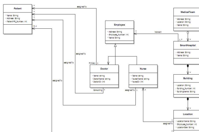
Figure 6(b): Class diagram for Asset Assignment
