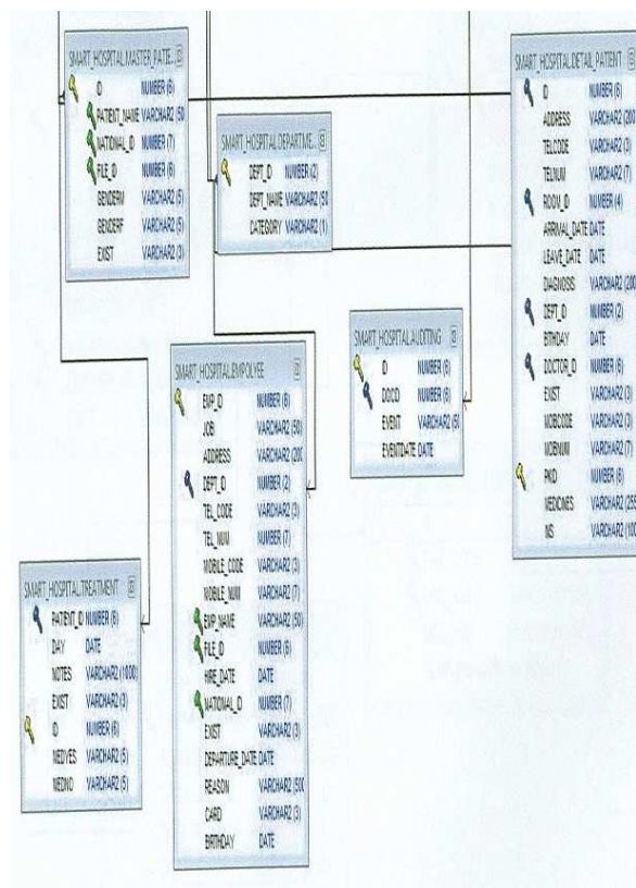
Figure 3b: Smart Hospital Schema 2
