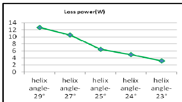
Figure 11. Power Loss at various at various Tip Relief
