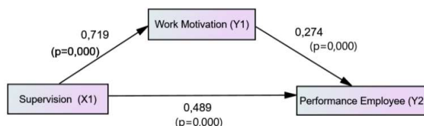
Figure 2. Result of Structural Equation Modeling
