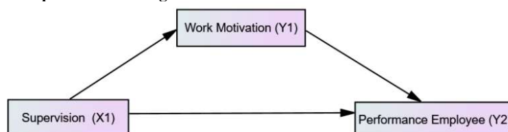
Figure 1. Structural Equation Modeling
