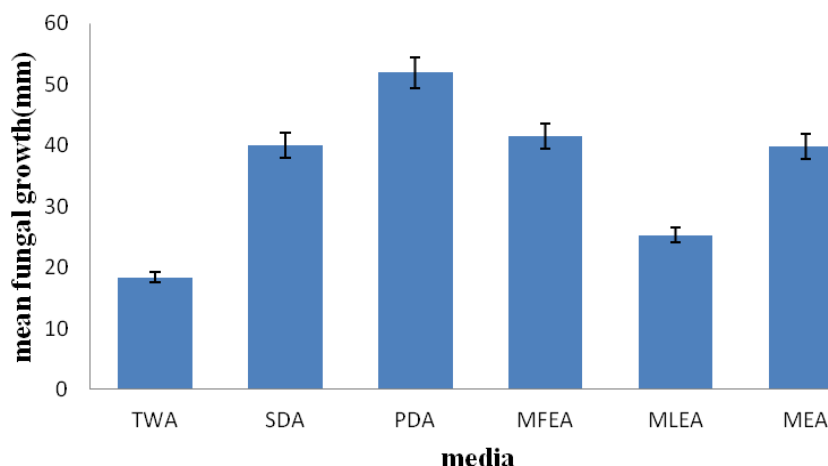
Figure 2. Mean mycelia growth of Colletotricum species on different media. Where, TWA= Tap water agar; SDA= Sabouraud dextrose agar; PDA= Potato dextrose agar; MLEA= Mango leaf extract agar; MFEA= Mango fruit extract agar and MEA= Malt extract agar
