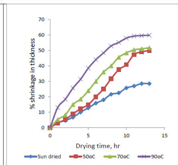
Fig 2(a) Effect of drying temperature and time on % shrinkage in the of blanched cylindrical thickness shaped 4mm thick sweet potato samples
