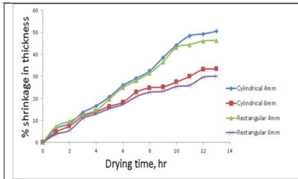
Fig 2(b) Effect of sample shape and thickness and drying time on %shrinkage in thickness of un-blanching sweet potato samples dried at 50°C
