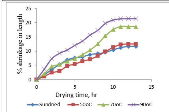
Fig 3(a) Effect of drying temperature and time on % shrinkage in sample length of unblanched rectangular shaped 6mm thick sweet potato samples
