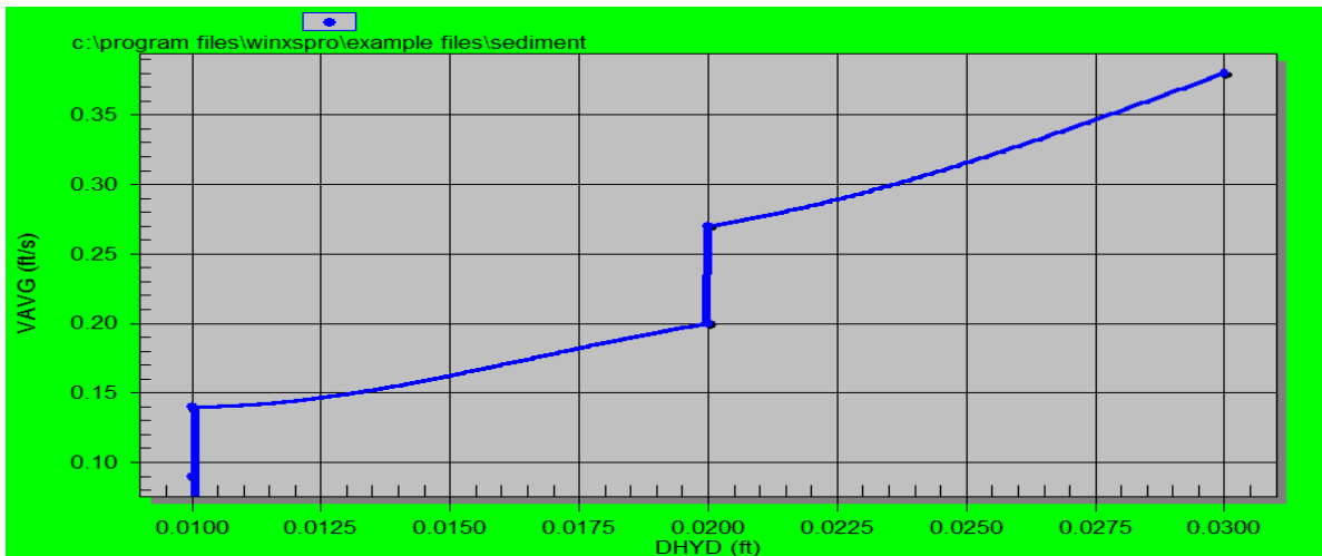
Figure 11: Avg. Velocity – Hydraulic Radius Relationship
