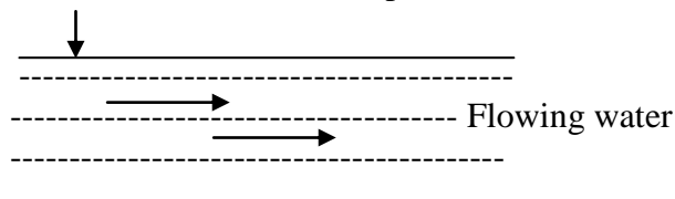
Figure 5: Flat Surface
