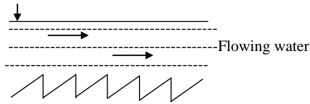
Figure 2: Saw-tooth Ripples
