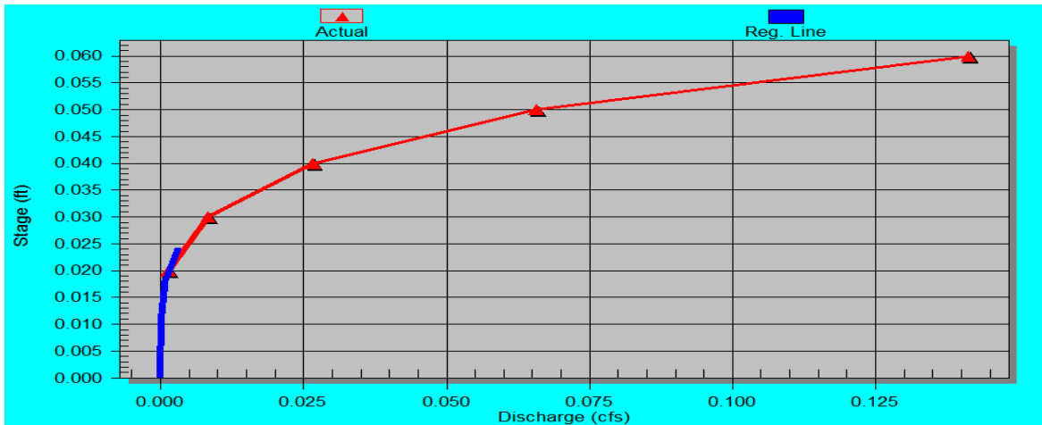
Figure 9: Stage – Discharge Relationship
