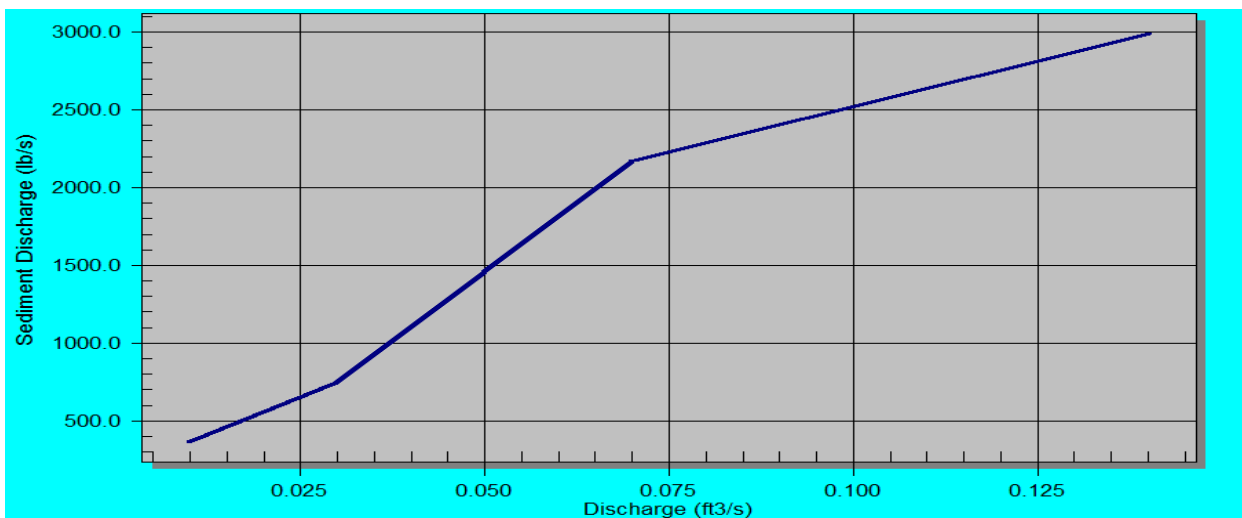
Figure 13: Sediment Discharge Function Relationship
