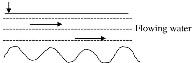
Figure 4: Dunes
