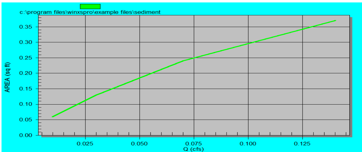
Figure 12: Area– Discharge Relationship
