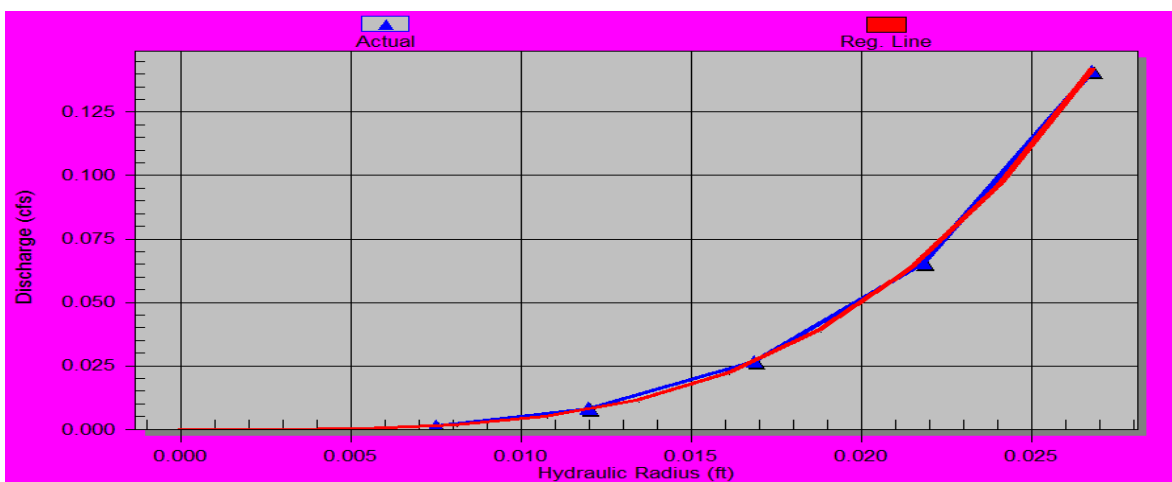
Figure 10: Discharge – Hydraulic Radius Relationship
