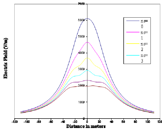
Fig. 6: Electric field distribution at 1m height above ground surface of the homopolar line with S=6m and H_s=15m
