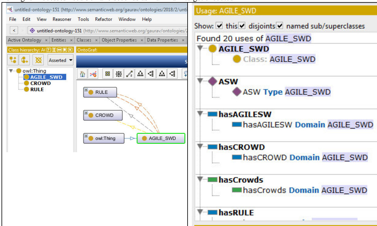
Figure no 4a: Basic Rule Ontology
