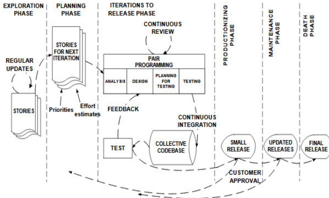
Figure no 1: XP Programming in Agile
