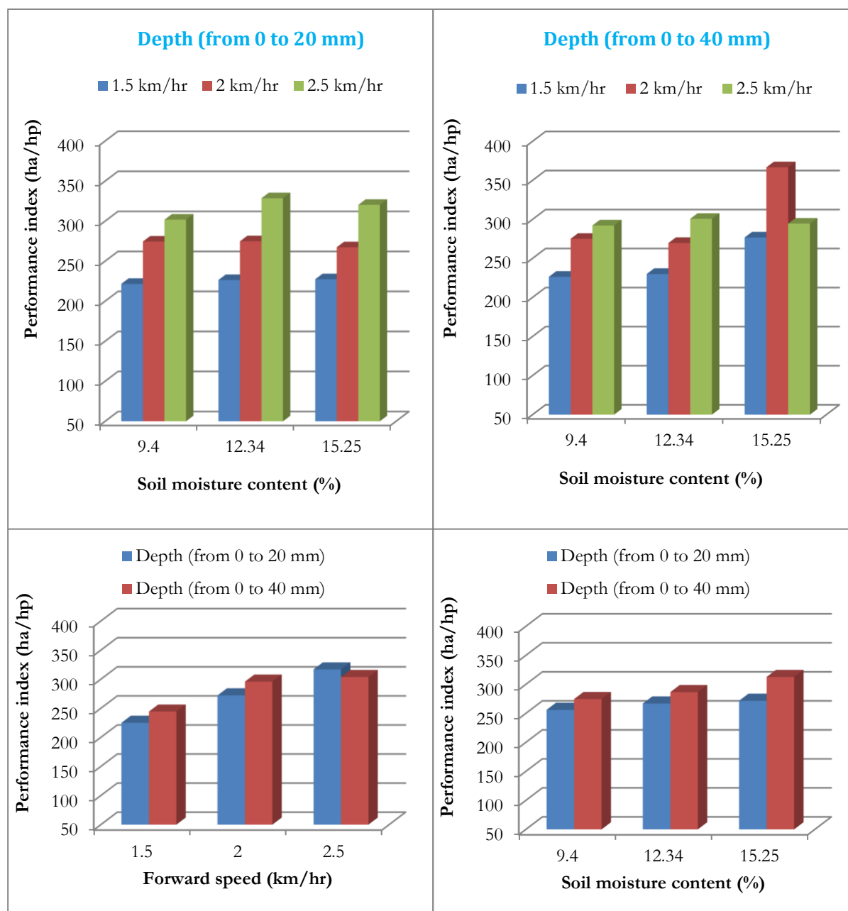
Figure 7: Effect of soil moisture and machine operational parameters on a performance index
