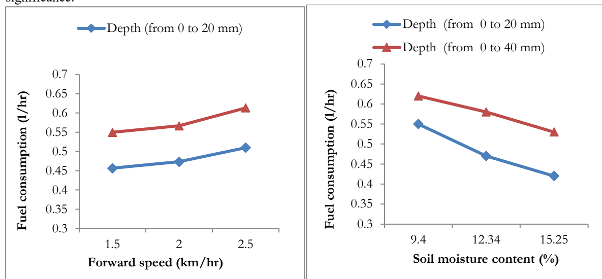
Figure 6: Effect of soil moisture and machine operation parameter on fuel consumption
