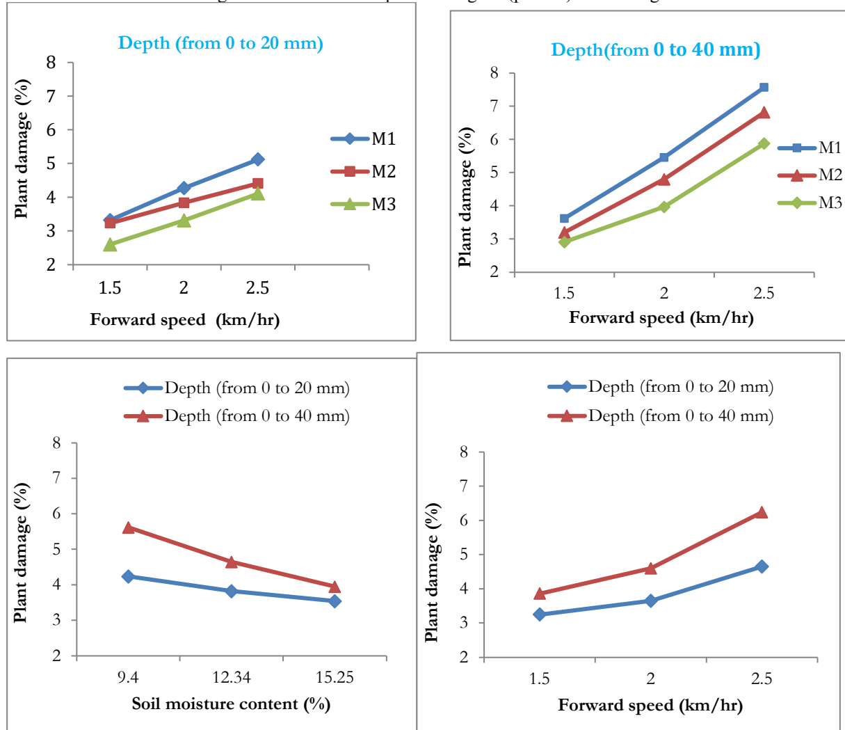
Figure 3: Effect of soil moisture and machine operational parameters on plant damage
