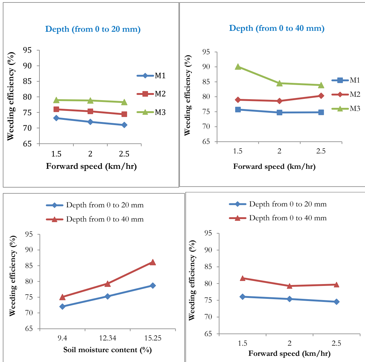
Figure 2: Effect of soil moisture and machine operational parameter weeding efficiency
