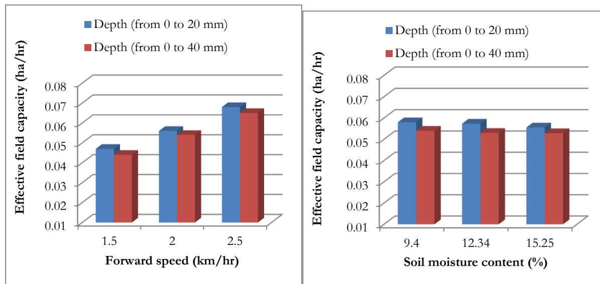
Figure 4. Effect of soil moisture and machine operational parameter on effective field capacity
