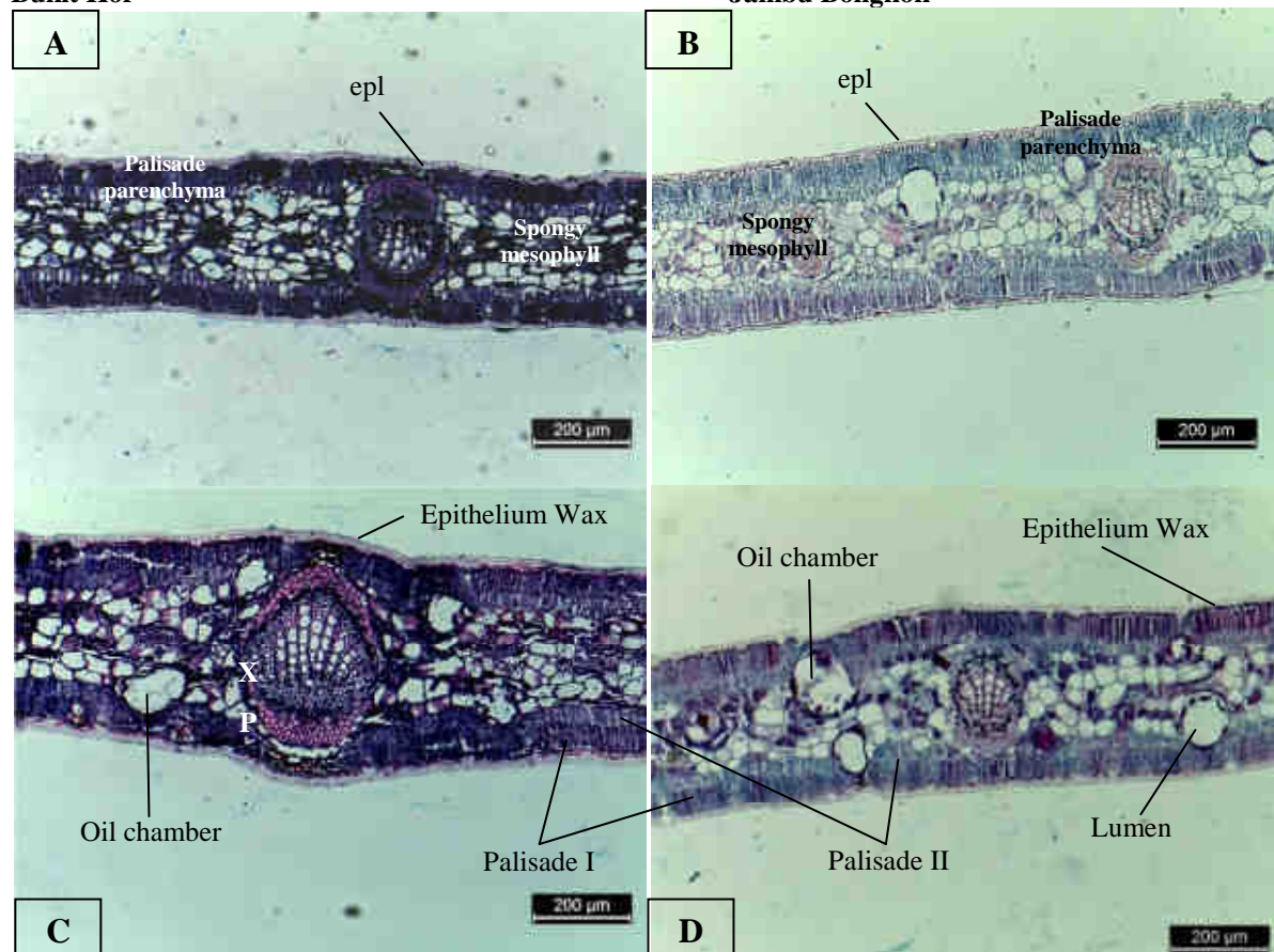
Figure 1. Comparative leaf anatomy in blade cross-sections of Gelam ( M. cajuputi Powell) leaves grown under a hard top soil area (A, C) and a large swamp forests, prominent flooding site (B, D) conditions. Epithelium wax in Bukit Kor is thicker compare to Jambu Bongkok. Vascular bundle are bigger in size in A & C. (Magnification 10X) (epl, epidermis layer; x, xylem; p, phloem; cw, cuticle wax; ml, middle lamella; oil, oils; epi, epitelium).
