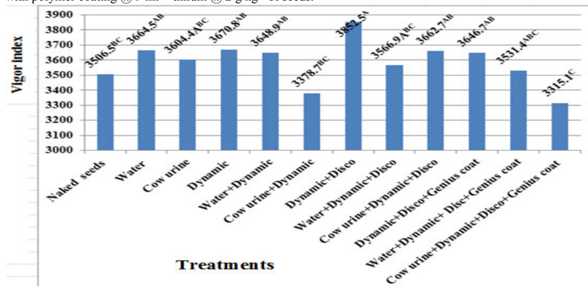
Fig 6: Effect of seed priming and coating treatments on bread wheat vigor index
