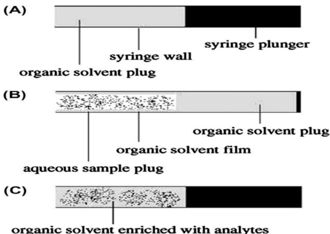
Fig 1. Operation of dynamic liquid-phase microextraction
