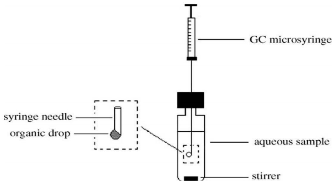
Fig 2. Direct-immersion single-drop microextraction
