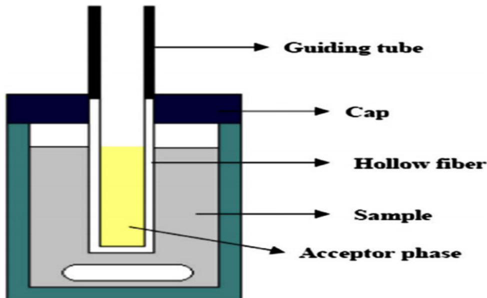
Fig 4. Principle of hollow-fiber liquid phase microextraction
