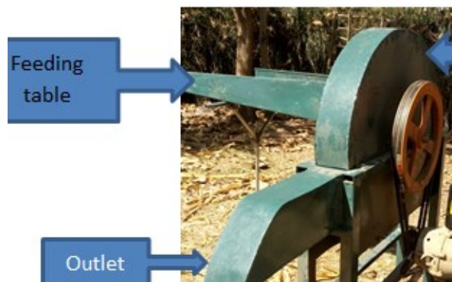
Figure 1. Chopper machine and main parts
