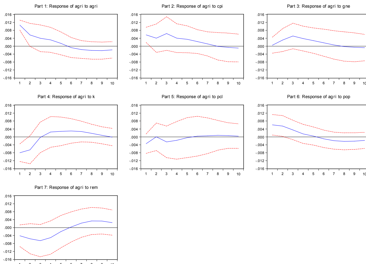
Figure 2: Response to Structural One S.D. Innovations \pm 2 S.E.
