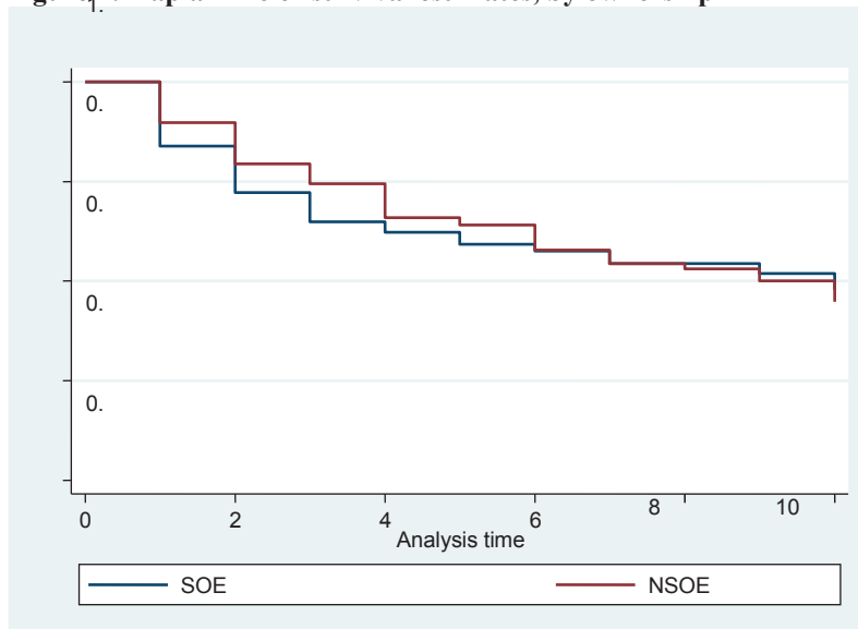
Figure 4: Kaplan-Meier survival estimates, by ownership
