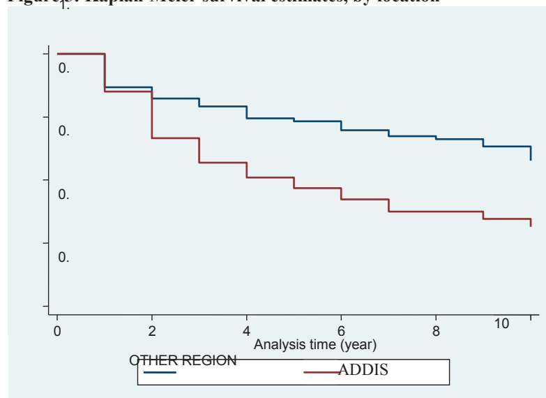
Figure 5: Kaplan-Meier survival estimates, by location
