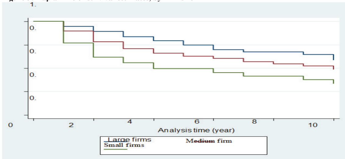
Figure 3: Kaplan-Meier survival estimates, by firm size
