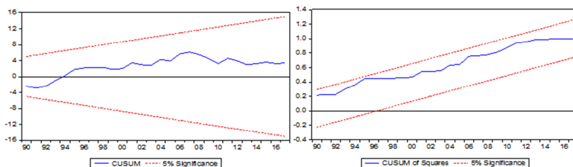
Figure 4.1: Plot of Cumulative sum of recursive residuals for Economic Growth
