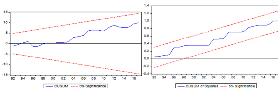
Figure 4.2: Plot of Cumulative sum of recursive residuals for Savings Model
