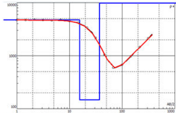
Fig. 2.1 :VES Curves and Layers Resistivity for Ukpulegbe (Ivue)
