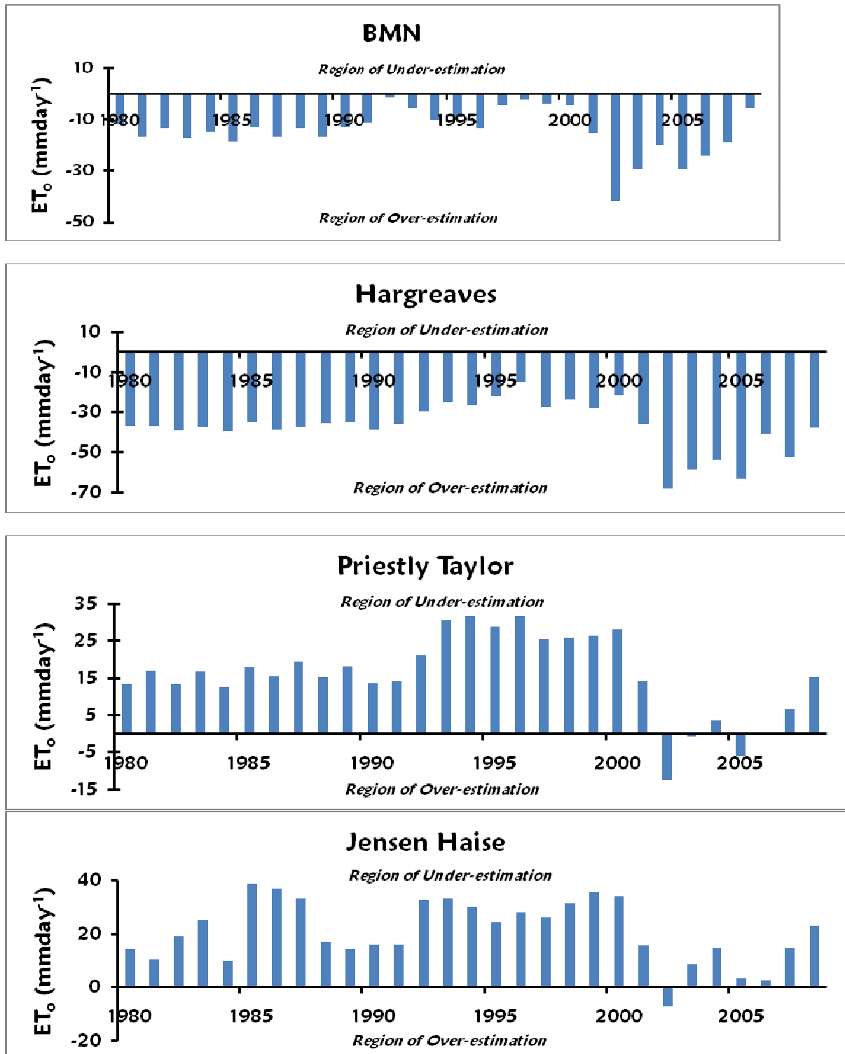
Figure 2: Annual Estimation difference between FAO56-PM ET_o values and the values from the other Models for Kano.
