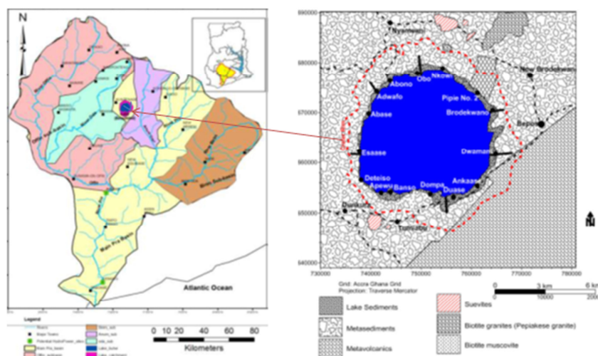
Figure 1. Map of the Pra river basin of Ghana showing the location of the Bosomtwi Crater Lake and the Geological profiles Bosomtwi crater area (Modified from Koeberl and Reimold 2005)
