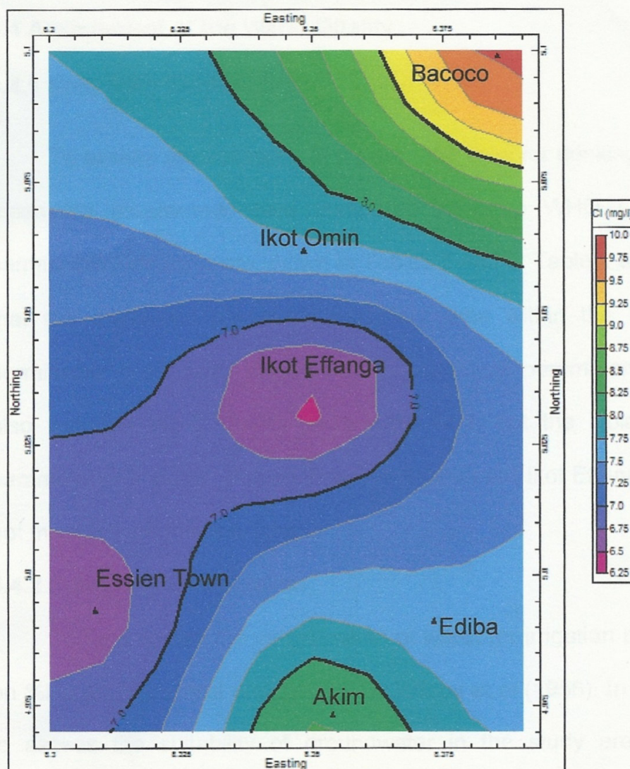
FIG.12: Distribution Pattern of Cl in the area.
