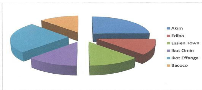
FIG.5: Pie chart comparing the concentration of Mg in the area.
