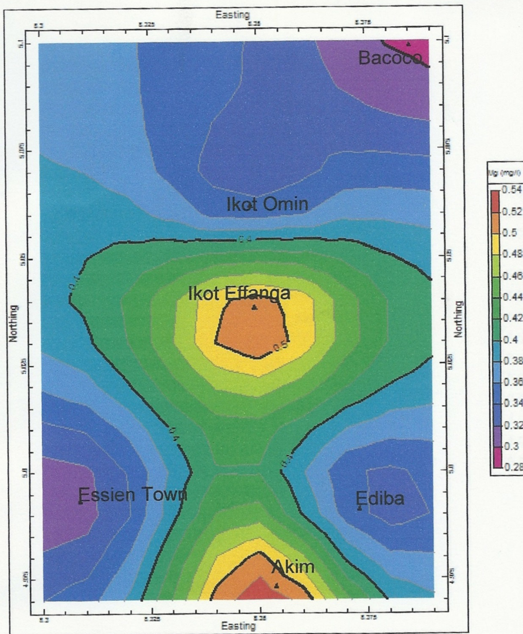
FIG.9: Distribution pattern of Mg in the area
