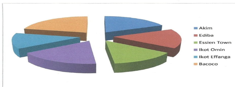
FIG.7: Pie chat showing the concentration of Cl in the area
