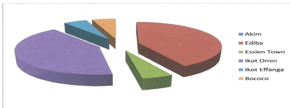
FIG.6: Pie chart comparing the concentration of \text{SO}_4 in the area.
