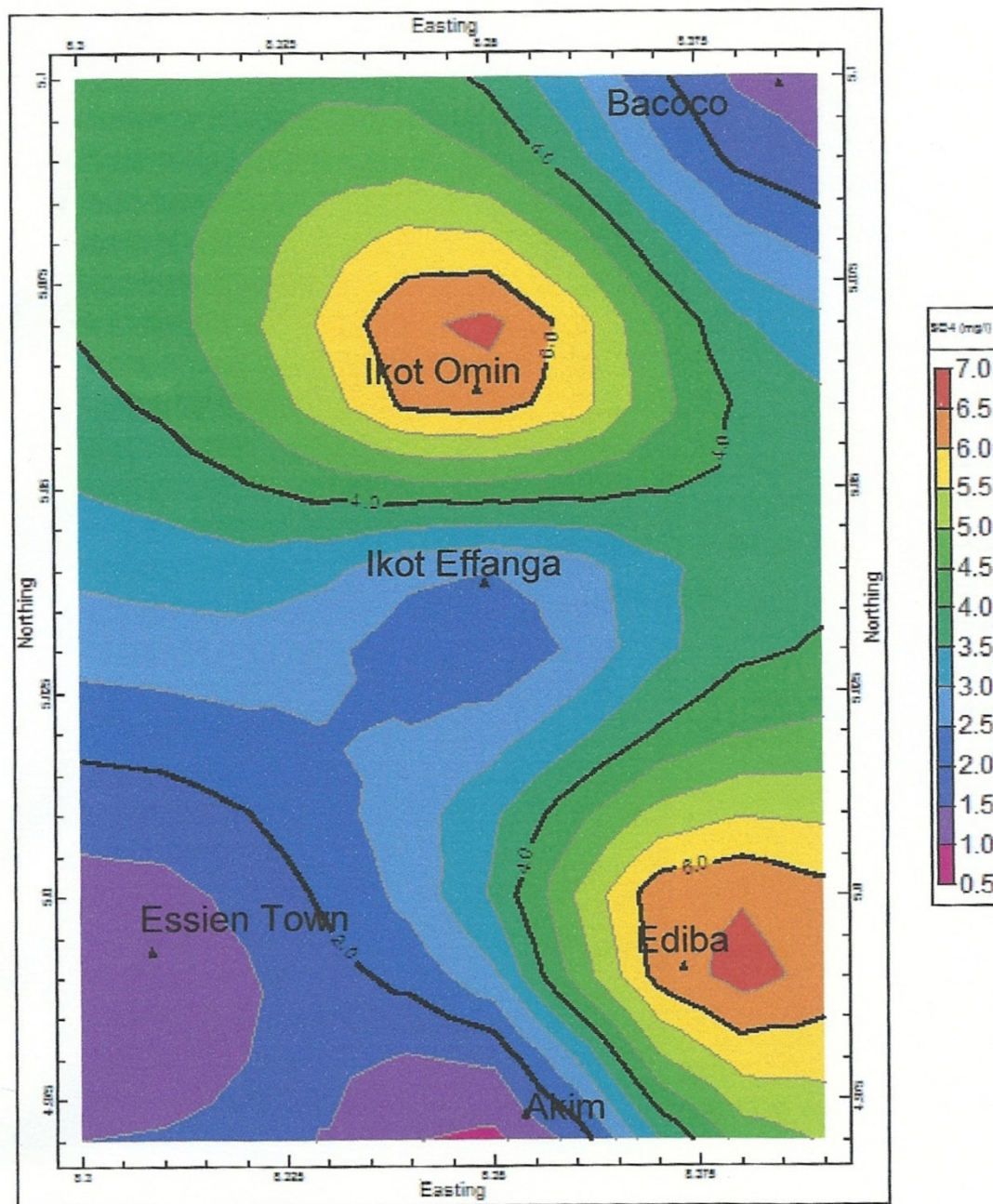
FIG. 10: Distribution Pattern of \text{SO}_4 in the area
