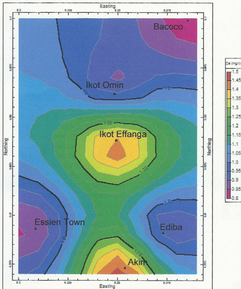
FIG.8 Distribution Pattern of Ca in the area
