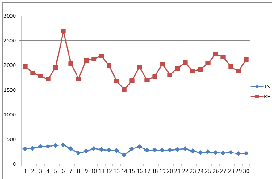
Figure 2: Annual Occurrence of Thunderstorm and Rainfall over Nigeria (1970-1990).
