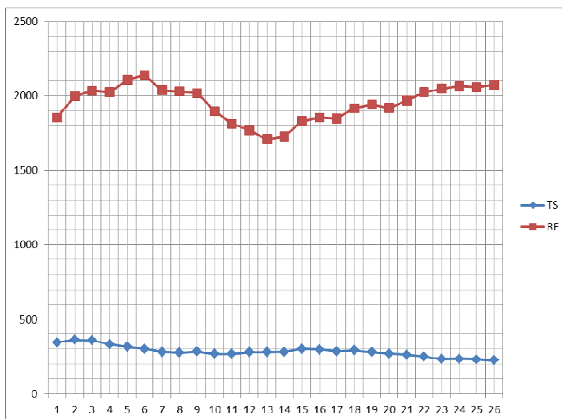
Figure3: The Running Mean of TS and RF (1970-1999).
