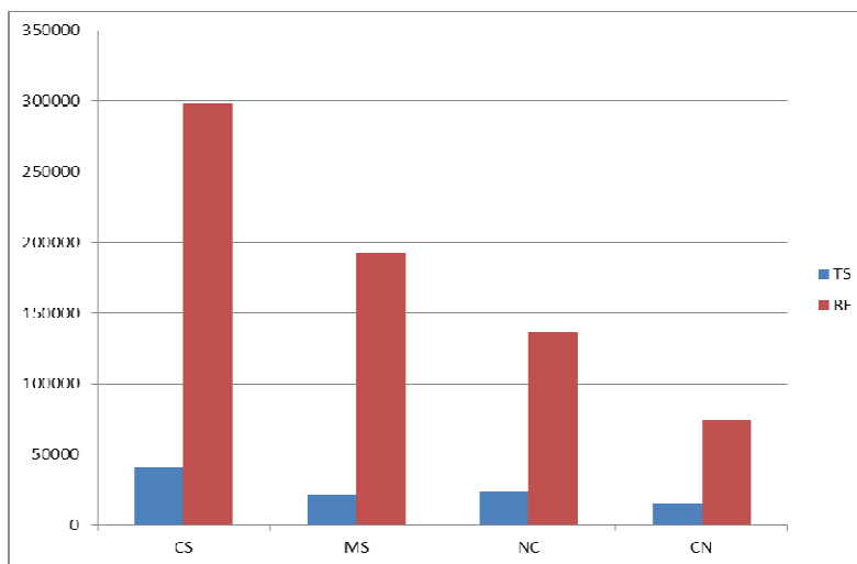
Figure4: Spatial Occurrence of TS and RF over Nigeria (1970-1999).
