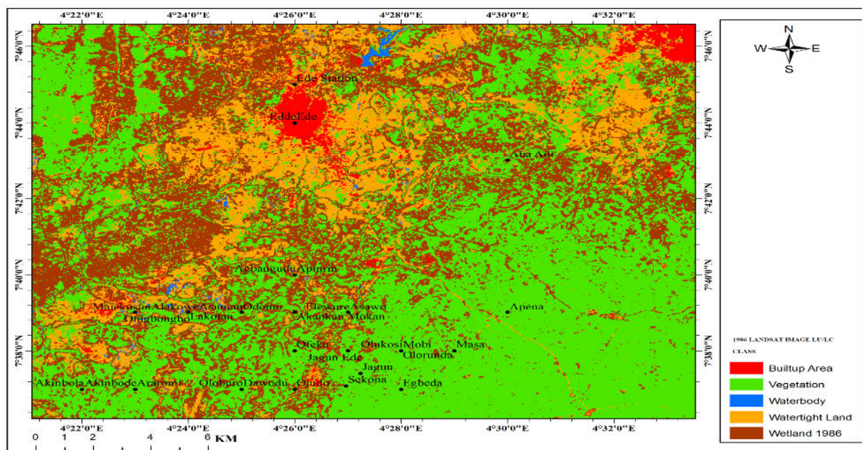
Fig. 3 1986 Image Classification of the study area
