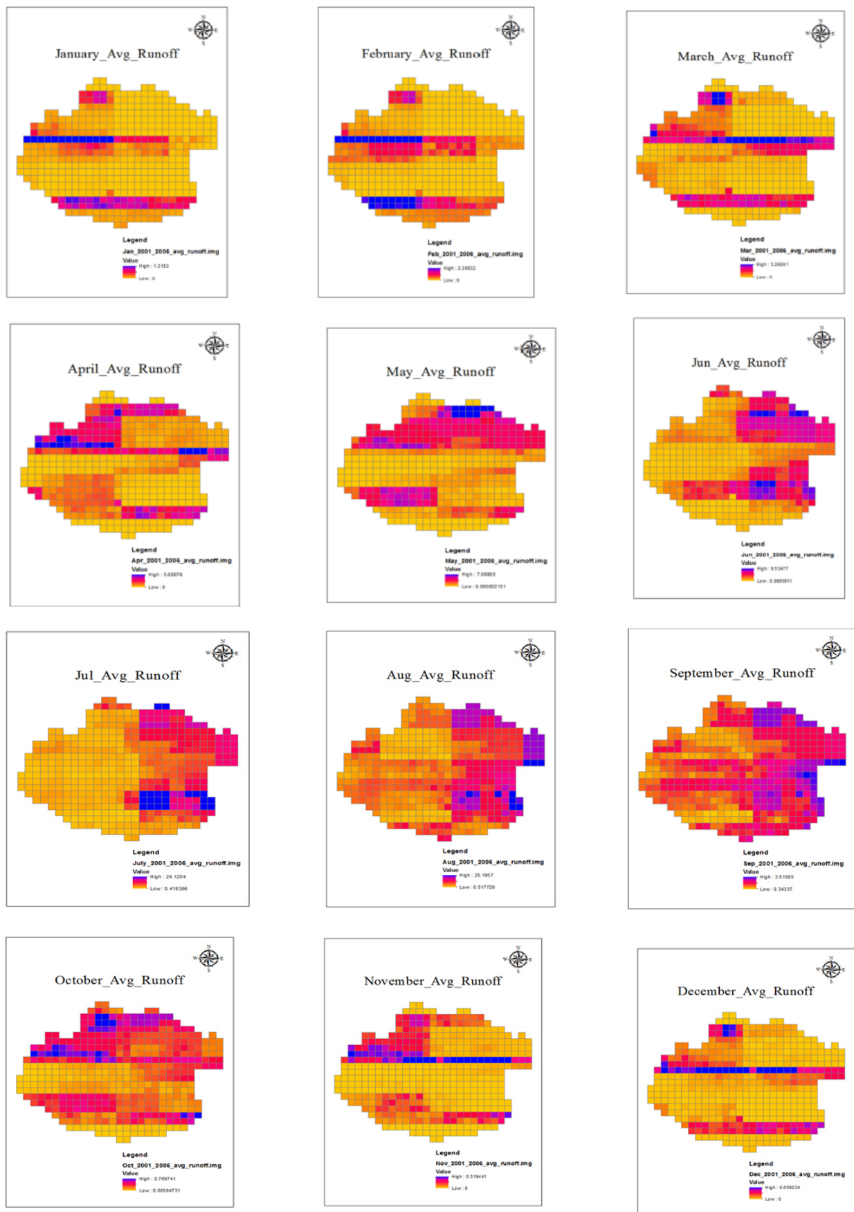
Fig. 6 Gridded Image of Runoff for Alaknanda River Basin Figure 6 indicates the runoff in the gridded image format generated by a Java programme from the VIC
