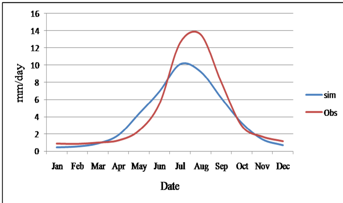
Fig. 4 Modeled and measured monthly average Discharge for Alaknanda River Basin
