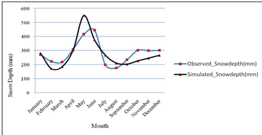
Fig. 7 Modeled and measured monthly average Snow Depth for Alaknanda River Basin
