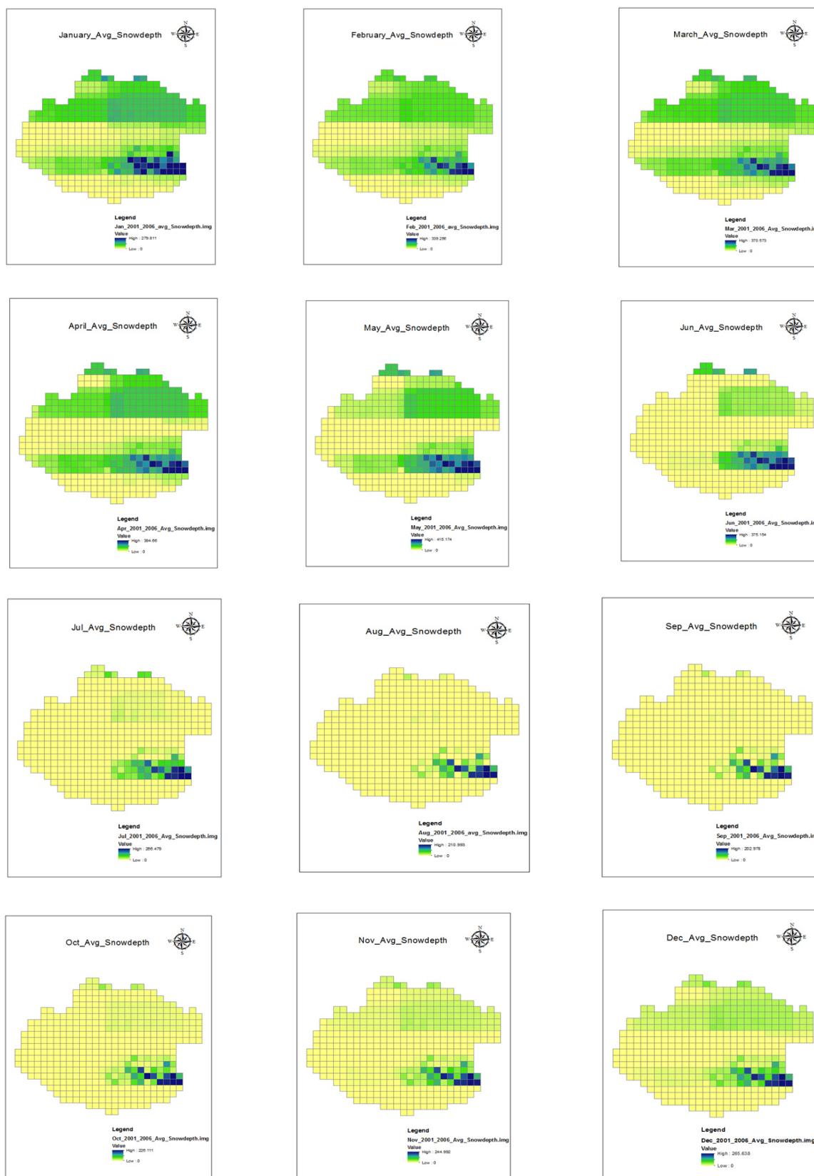
Fig. 9 Gridded Image of Snow Depth for Alaknanda River Basin
