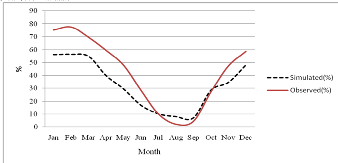
Fig. 10 Modeled and measured monthly average snow cover fraction
