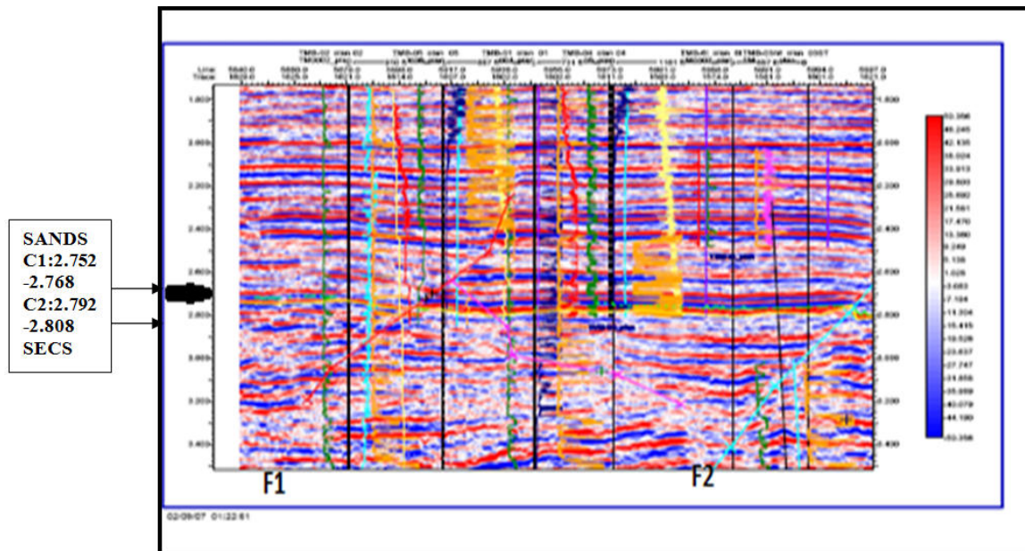
Figure 2. ‘X’-Field, Niger Delta: Arbitrary line after interpretation: Two major faults ,F1,F2 are shown bounding the wells at the reservoir interval under analysis (2.752-2.768 secs).The well locations are indicated
