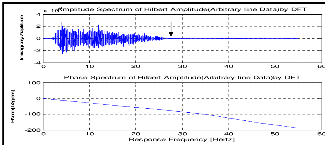
(c)Base of Reservoir (2.768 s):Amplitude and Phase Spectra of Arbitrary line by Hilbert Transform (HT)
