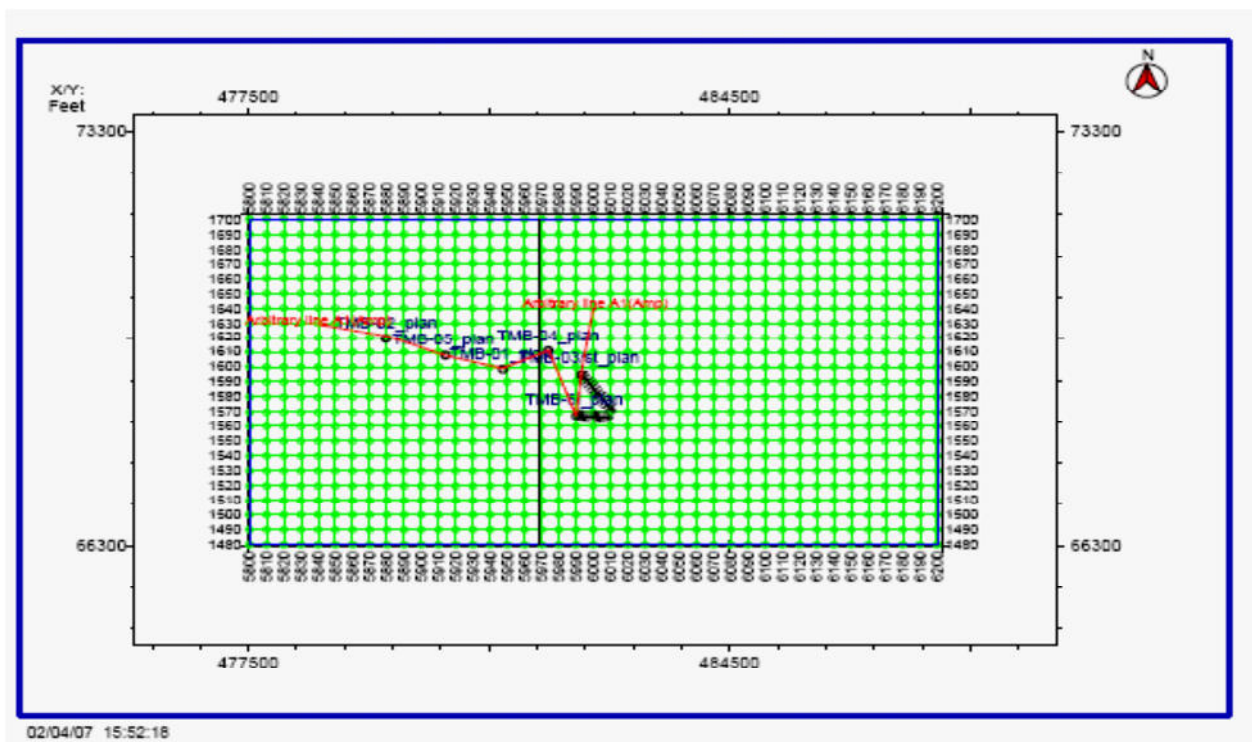
Figure 1: 'X'-Field, Niger Delta. : Base map of survey area showing the arbitrary line (red). The Arbitrary line connects the entire wells (six) in the survey.
