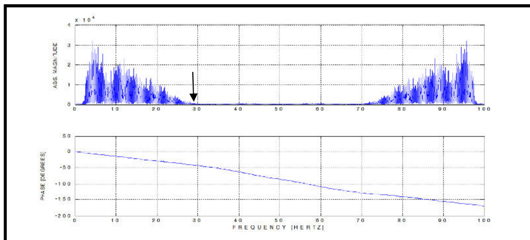
(a)Top of Reservoir(2.752 s): Amplitude and Phase Spectra of original Arbitrary line data by Discrete Fourier Transform (DFT)
