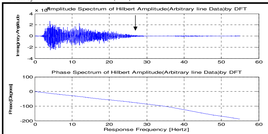
(b)Top of Reservoir (2.752 s): Amplitude and Phase Spectra of Arbitrary line by Hilbert transform (HT)
