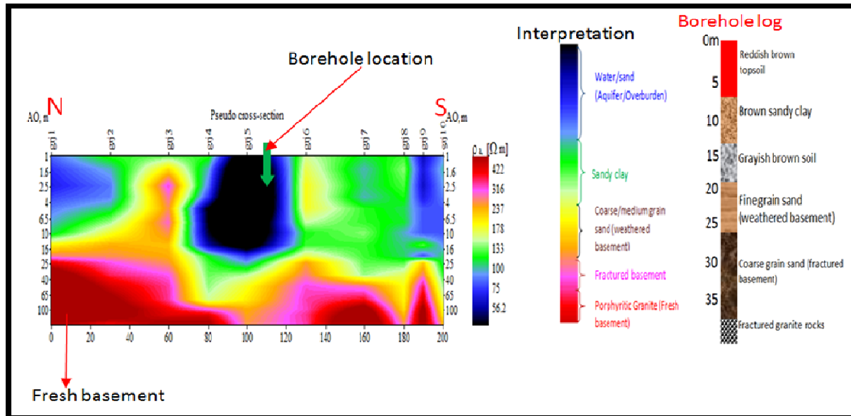
Figure6: Resistivity tomography section for Garaje Profile.
