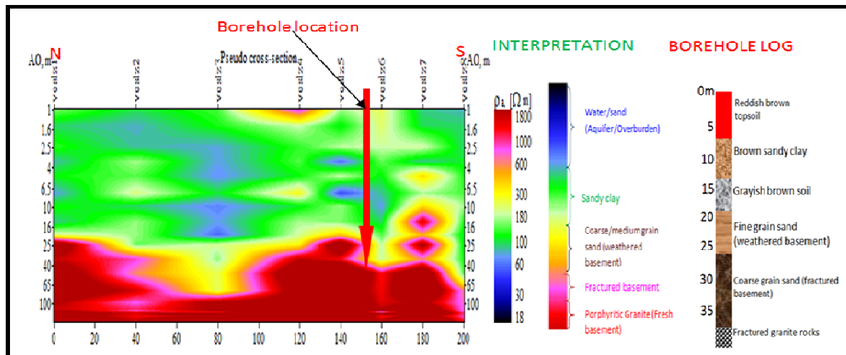
Figure7: Resistivity tomography section for LGEA Zakwa Profile
