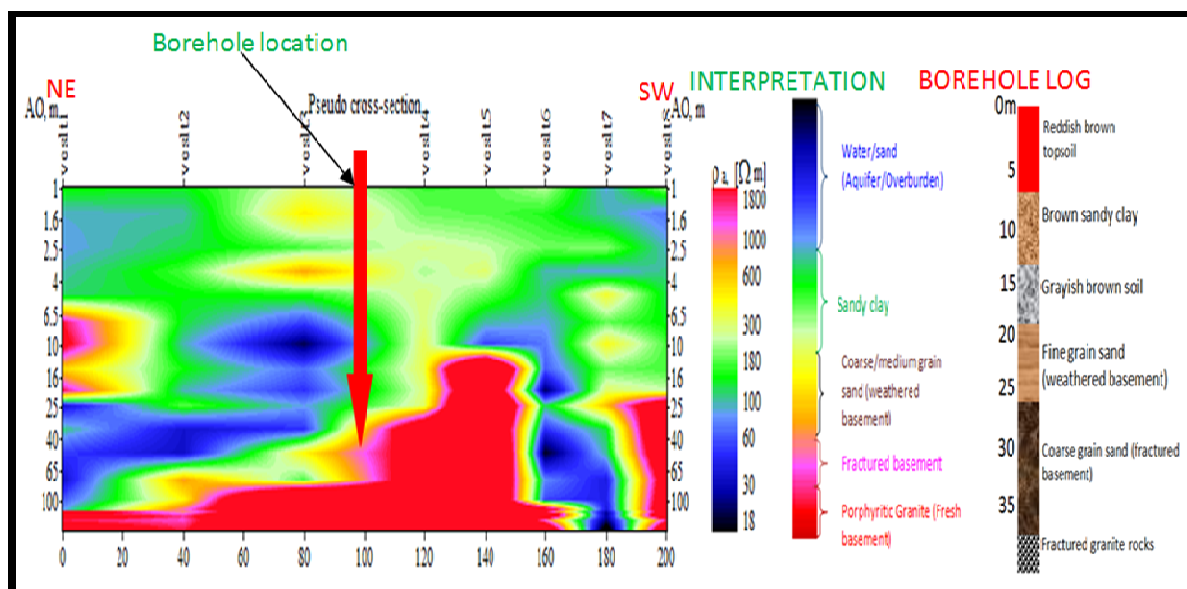
Figure8: Resistivity tomography section for LGEA Techarak Profile
