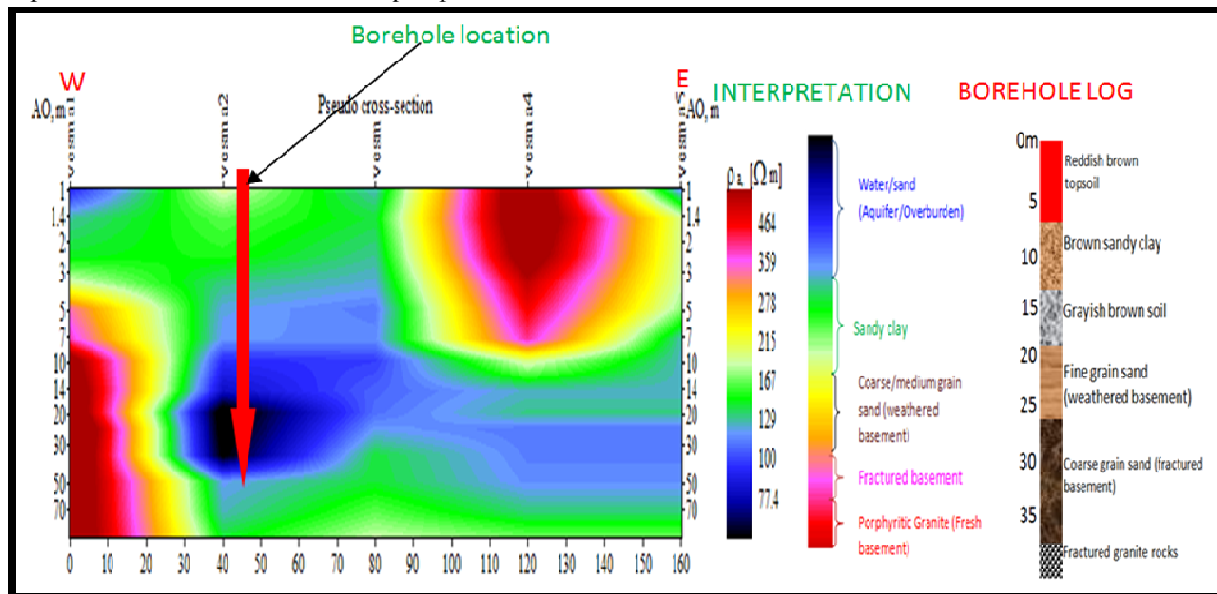
Figure9: Resistivity tomography section for LGEA Madamai Profile
