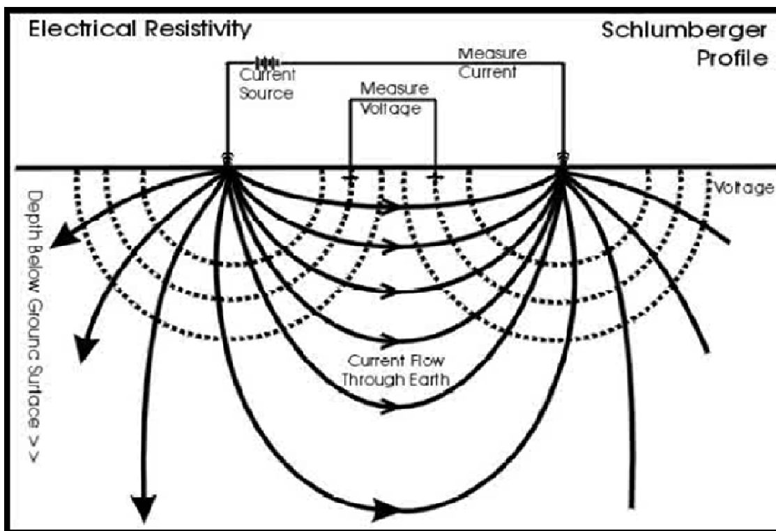
Figure4. The Full-Schlumberger Array
